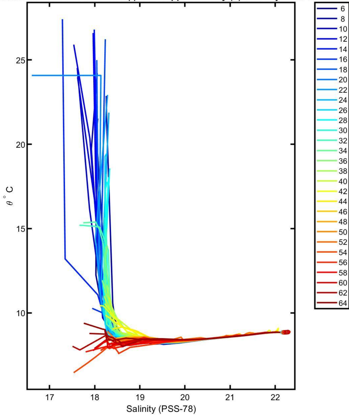
7900593 uncalibrated float data (-) and mapped salinity (o) with objective errors
