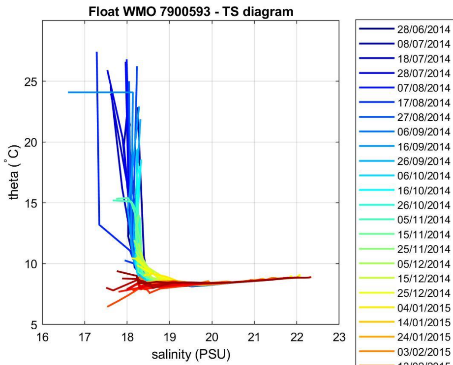
Figure 3: Float 7900593. \theta -S diagram color-coded per cycle number.
