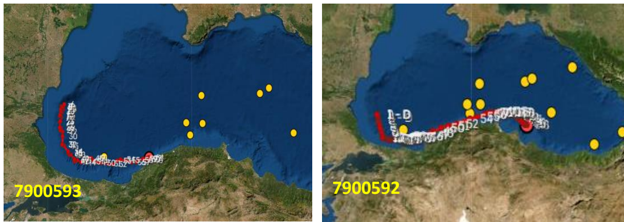
Figure 19: Float 7900593. Trajectory of the floats used for the comparison.
