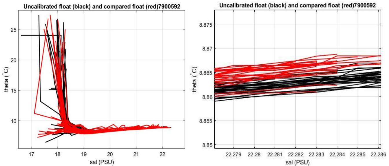
Figure 20: Float 7900593. Comparison between float 7900593 (black line) and 7900592 (red line), in the most uniform part of the \theta -S curve.
