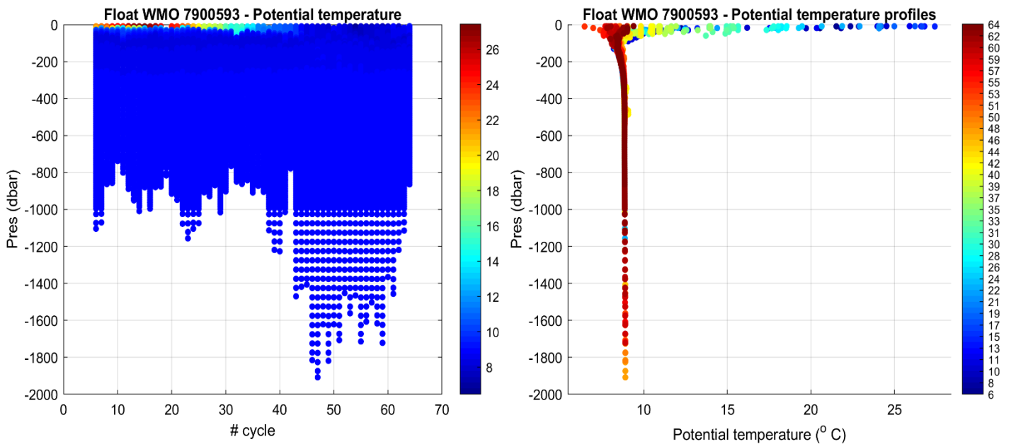
Figure 1: Float 7900593. Time series of Argo float potential temperature ( ^{\circ}\text{C} ) on the left, and potential temperature profiles color-coded per cycle number on the right.
