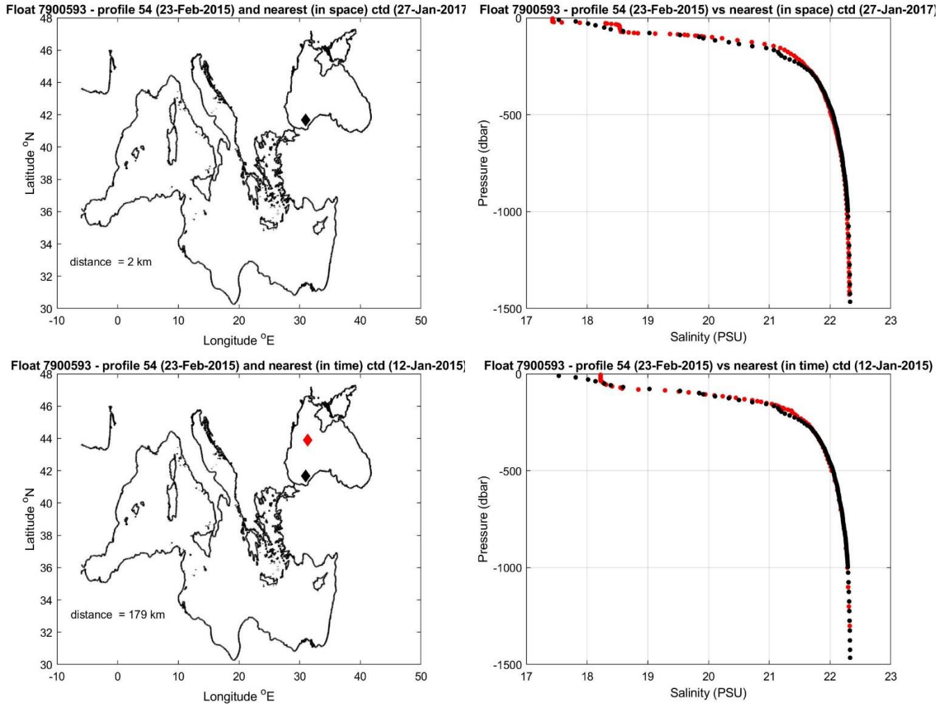
Figure 10: Float 7900593. The salinity float profile number 54 (black dots) are compared to the nearest in space (top) and in time (bottom) reference profile (red dots). The locations of the two profiles and their distance is given in the left panel.
