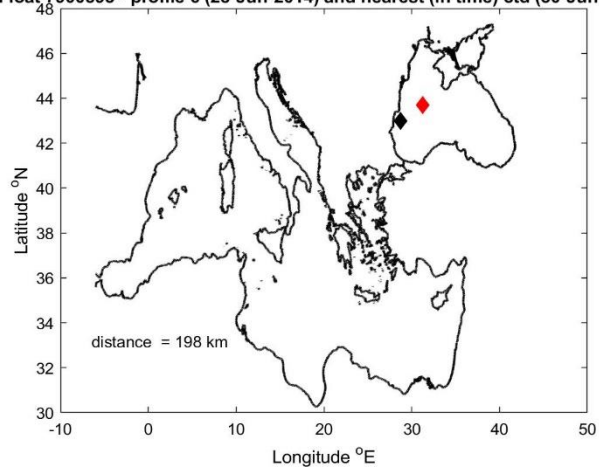
Float 7900593 - profile 6 (28-Jun-2014) and nearest (in time) ctd (30-Jun-2014)
