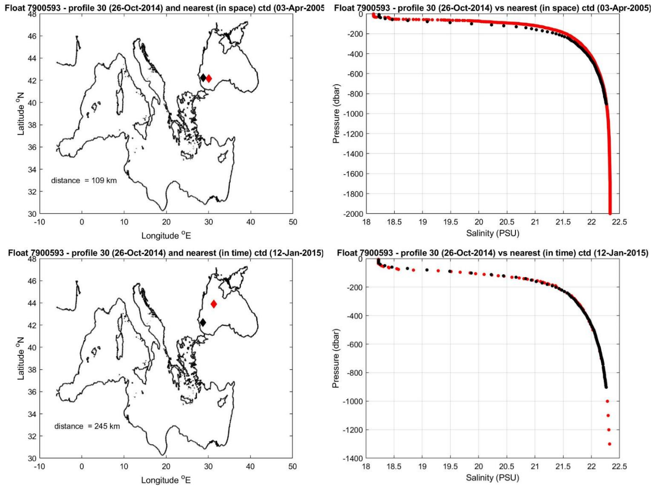
Figure 9: Float 7900593. The salinity float profile number 30 (black dots) are compared to the nearest in space (top) and in time (bottom) reference profile (red dots). The locations of the two profiles and their distance is given in the left panel.
