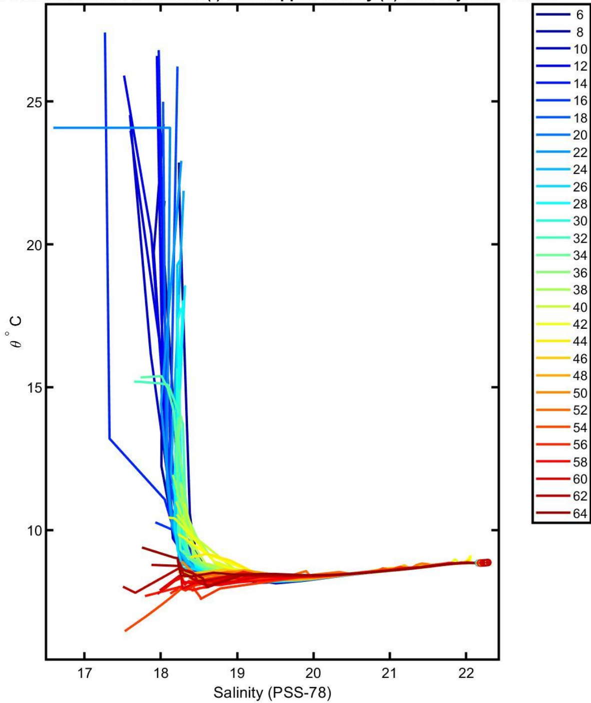
7900593 calibrated float data (-) and mapped salinity (o) with objective errors
