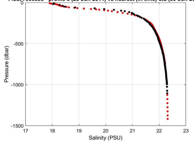
Float 7900593 - profile 6 (28-Jun-2014) vs nearest (in time) ctd (30-Jun-2014)
