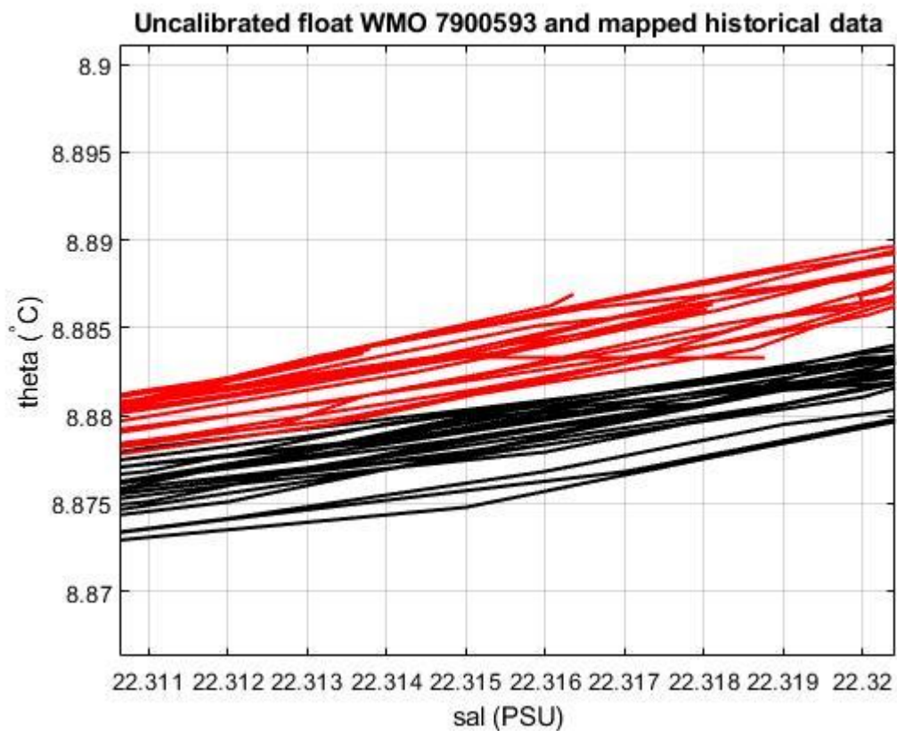
Figure 18: Float 7900593. Uncalibrated float salinity profile (black lines) and mapped historical data (red lines) in the most uniform part of the \theta -S curve.
