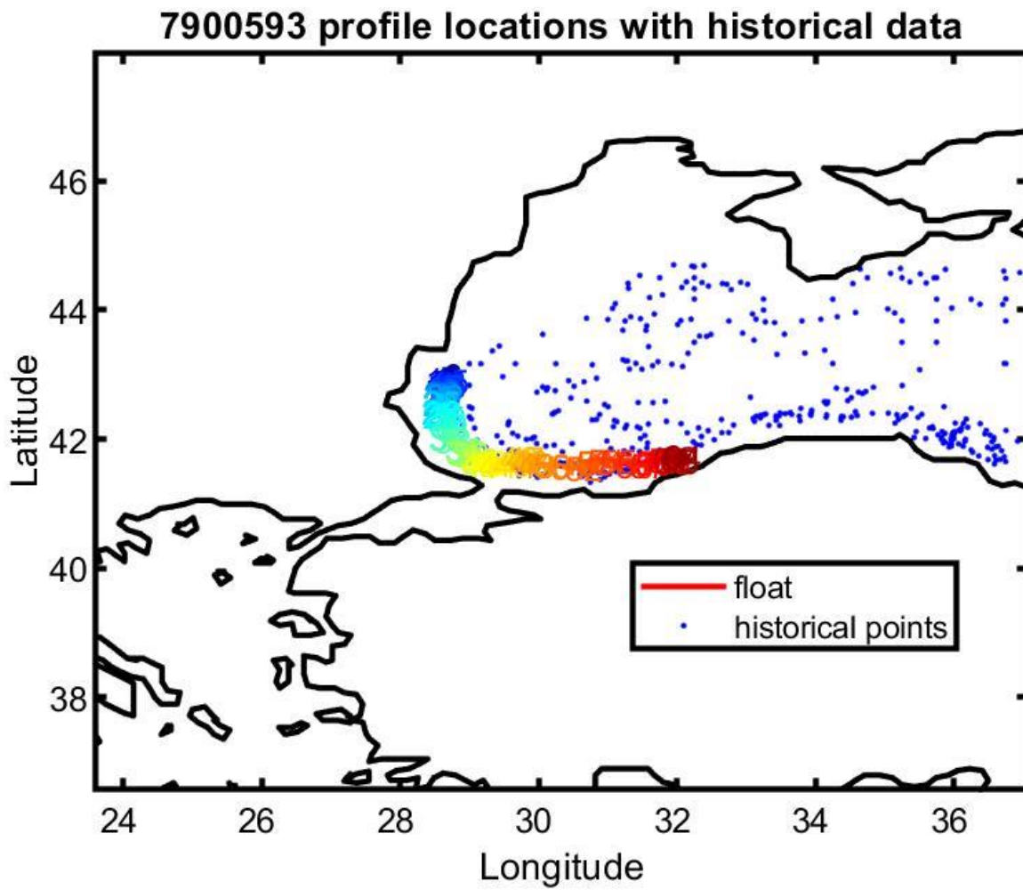
Figure 12: Float 7900593. Location of the float profiles (red line with colored numbers) and the reference data selected for mapping (blue dots).
