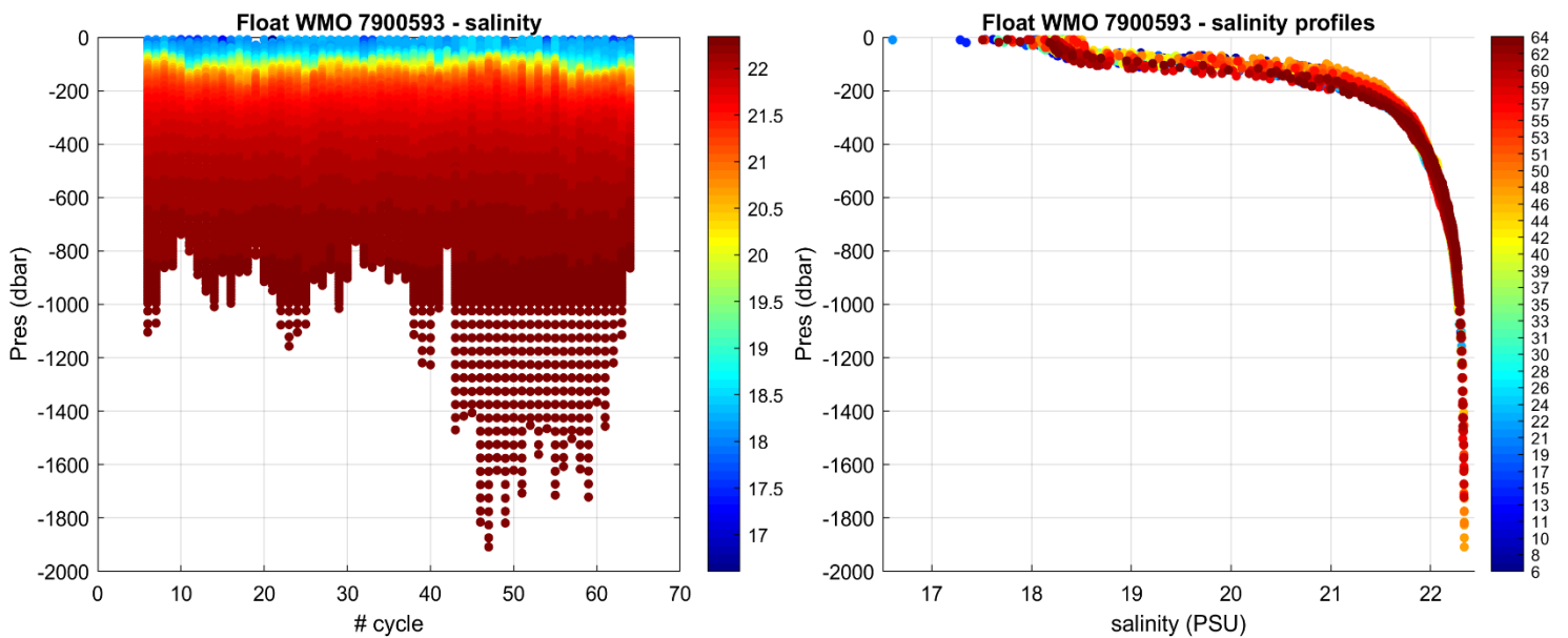
Figure 2: Float 7900593. Time series of Argo float potential salinity (PSS-78) on the left, and salinity profiles color-coded per cycle number on the right.
