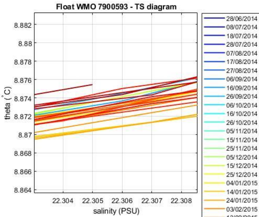
Figure 4: Float 7900593. Area of the \theta -S diagram (color-coded per cycle number) where the \theta -S relationship is more uniform.
